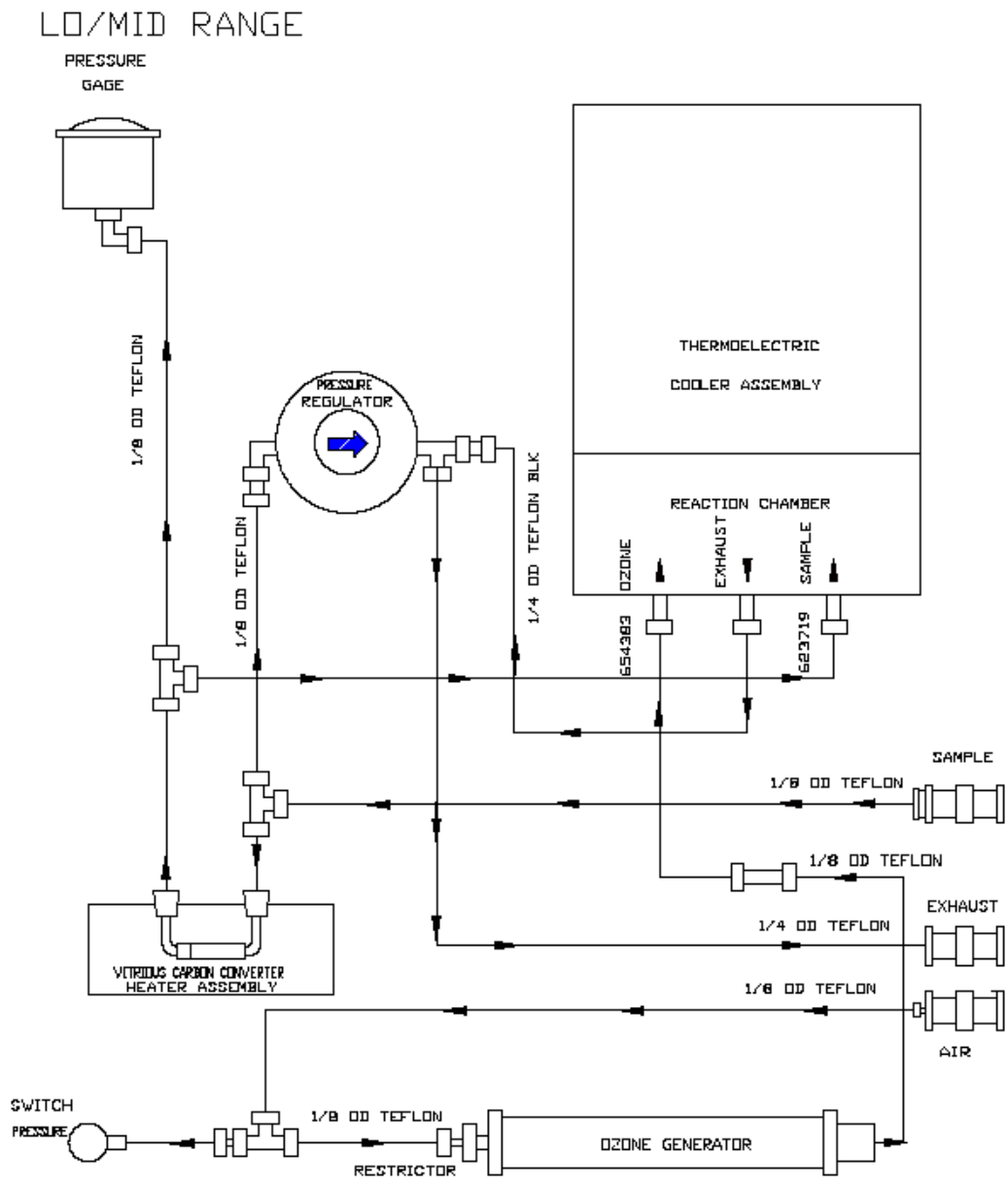
Drawing 1-2 Flow Diagram, Lo/Mid Range
